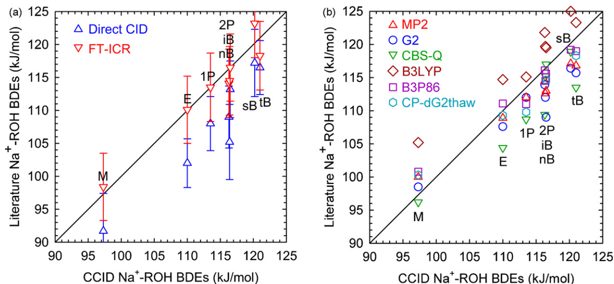
Fig. 4. Absolute 0 K Na^+-(ROH) bond dissociation energies determined by (a) direct CID (open triangles with error bars, Ref. [16]) and FT-ICR equilibrium studies (open inverted triangles with error bars, Ref. [4]) and (b) theoretical calculations at the MP2(full)/6-311+G(2d,2p)//MP2(full)/6-31G(d) (triangles, Ref. [16]), G2 (circles, Ref. [16] and present work), CBS-Q (inverted triangles, Ref. [16]), B3LYP/6-311+G(2d,2p)//B3LYP/6-31G(d) (diamonds, Ref. [2] and present work), B3P86/6-311+G(2d,2p)//B3P86/6-31G(d) (squares, Ref. [2] and present work), and CP-dG2thaw (hexagons, Ref. [7]) levels of theory versus competitive CID (CCID) bond dissociation energies from Table 2. The diagonal line indicates the values for which literature values are equal to the CCID values. M = MeOH, E = EtOH, 1P = 1-PrOH, 2P = 2-PrOH, nB = n -BuOH, iB = i -BuOH, sB = s -BuOH, tB = t -BuOH.
