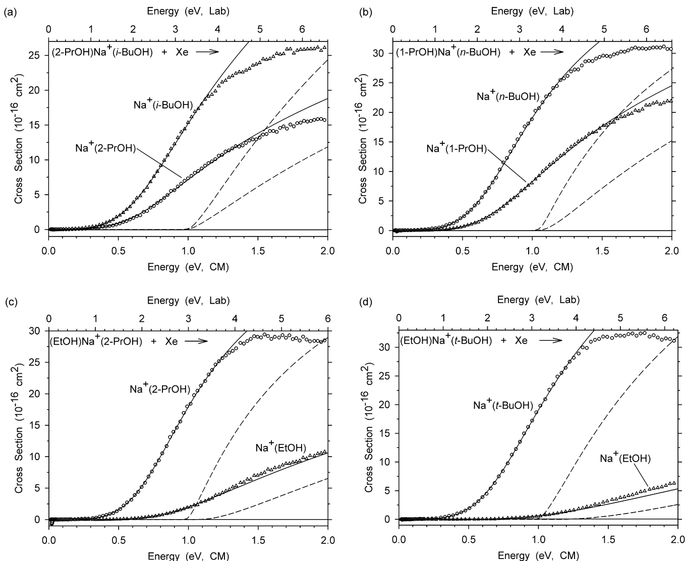
Fig. 2. Zero pressure extrapolated cross sections for the competitive collision-induced dissociation processes of (a) (2\text{-PrOH})\text{Na}^+(\text{i-BuOH}) , (b) (1\text{-PrOH})\text{Na}^+(\text{n-BuOH}) , (c) (\text{EtOH})\text{Na}^+(2\text{-PrOH}) , and (d) (\text{EtOH})\text{Na}^+(\text{t-BuOH}) with xenon in the threshold region as a function of kinetic energy in the center-of-mass frame (lower axis) and laboratory frame (upper axis). Solid lines show the best fits to the data using the model of Eq. (1) convoluted over the neutral and ion kinetic energies and the internal energies of the reactants. Dashed lines show the model cross sections in the absence of experimental energy broadening for reactants with an internal energy of 0 K.
