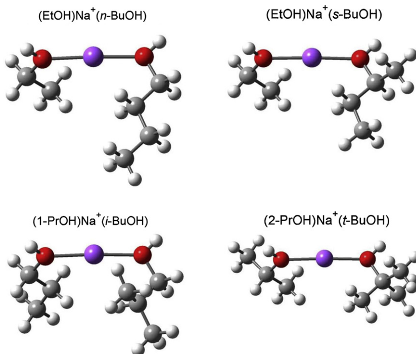
Fig. 3. Ground state geometries of (EtOH)Na + ( n -BuOH), (EtOH)Na + ( s -BuOH), (1-PrOH)Na + ( i -BuOH), and (2-PrOH)Na + ( t -BuOH) complexes, optimized at the MP2(full)/6-31G(d) level of theory.
