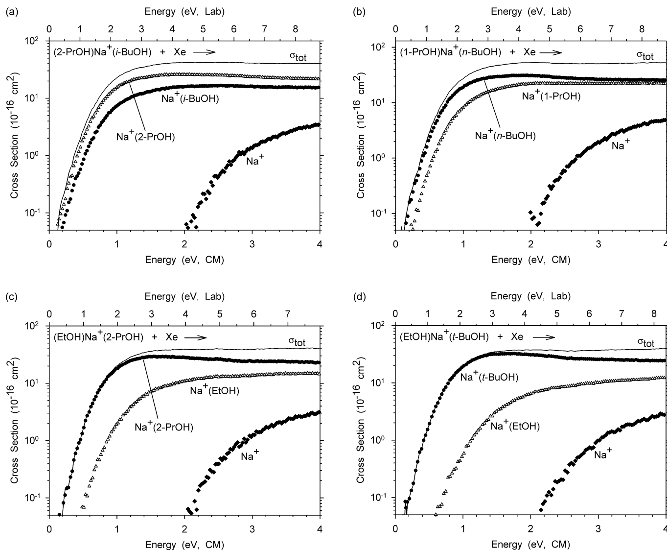
Fig. 1. Cross sections for collision-induced dissociation of (a) (2-PrOH)Na + (i-BuOH), (b) (1-PrOH)Na + (n-BuOH), (c) (EtOH)Na + (2-PrOH), and (d) (EtOH)Na + (t-BuOH) with xenon as a function of kinetic energy in the center-of-mass frame (lower axis) and laboratory frame (upper axis). Solid lines show the total cross section for each system and the symbols represent data extrapolated to zero pressure.
