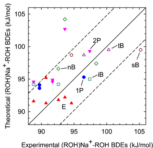
Fig. 5. Experimental versus theoretical absolute 0 K (R_1OH)Na^+-(R_2OH) bond dissociation energies, according to the R_2OH ligand: EtOH (E, closed triangles), 1-PrOH (1P, closed circles), n -BuOH (nB, open diamonds), i -BuOH (iB, open squares), 2-PrOH (2P, closed inverted triangles), s -BuOH (sB, open hexagons), and t -BuOH (tB, open triangles). All values are taken from Table 4. The solid diagonal line indicates the values for which measured and calculated values are equal. The dashed diagonal lines indicate an uncertainty of \pm 4.8 kJ/mol about the solid diagonal line.
